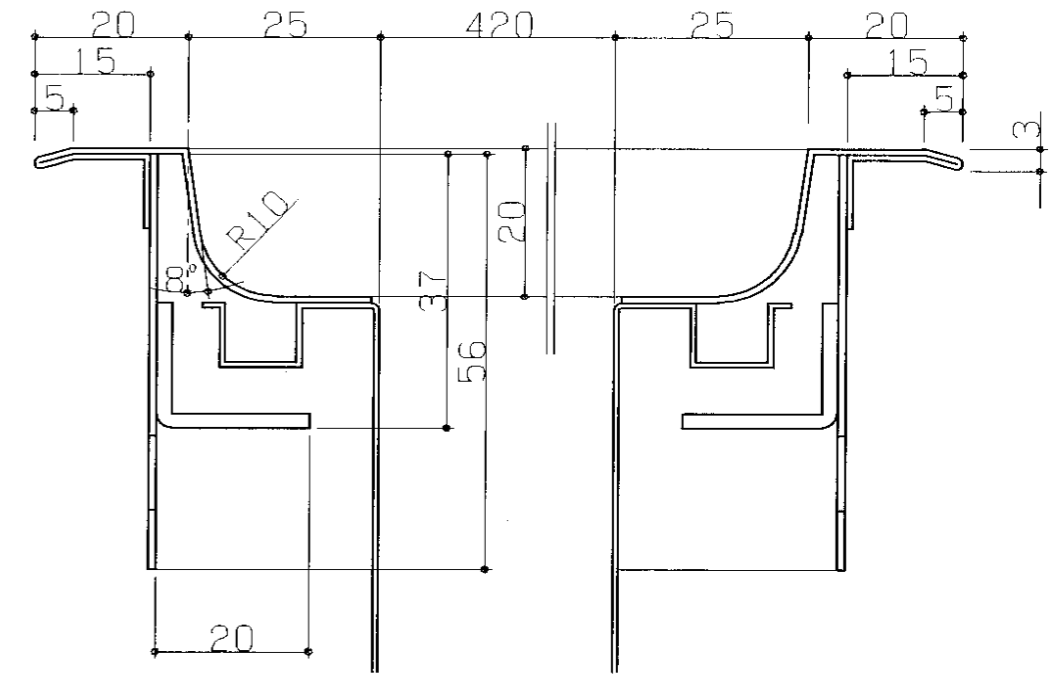
AA断面(1/1)
